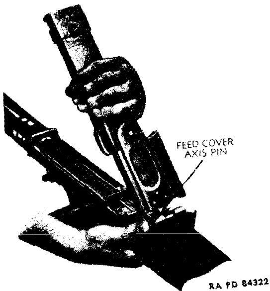
Figure 25 – Removal of Feed Cover
