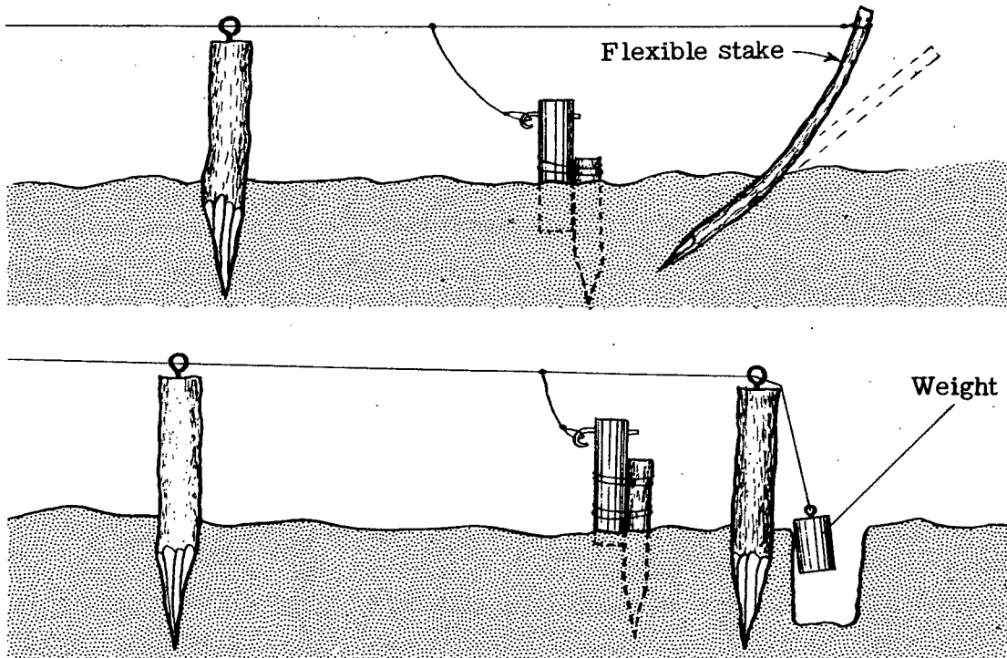
Figure 119. Use of grenade in trip-wire booby traps: Above, using a flexible stake to pull out the suspension wire; below, using a weight for the same purpose.
