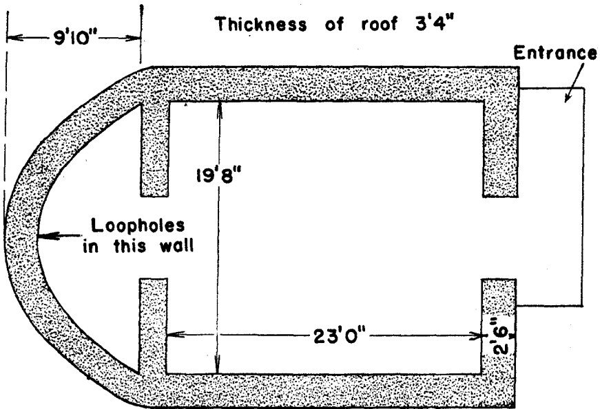
Figure 40.—Underground emplacement.
