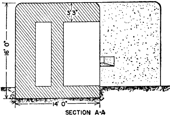
Figure 42.—Emplacement for two machine guns.
