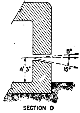
Figure 42.—Emplacement for two machine guns.
