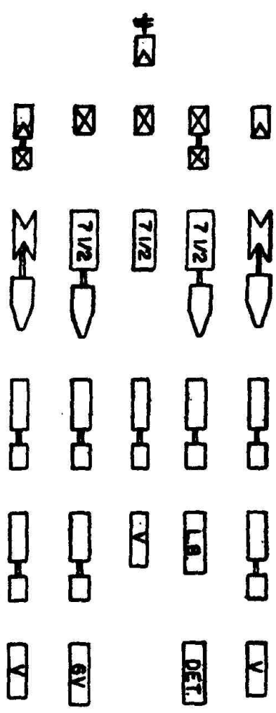
FIGURE 8.—Battery mass formation, mounted—90-mm gun battery.
