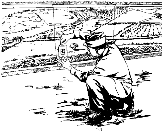
FIGURE 80.—Lining in scoring area (point target) with scoring template.
