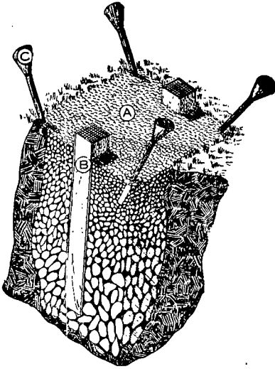
FIGURE 16.—Urine soakage pit.
