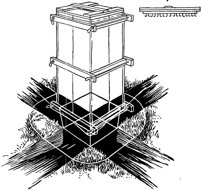
FIGURE 67.—Disinfestor, Serbian barrel, knock-down type.
