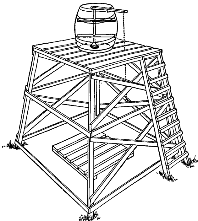
FIGURE 64.—Improvised shower bath.
