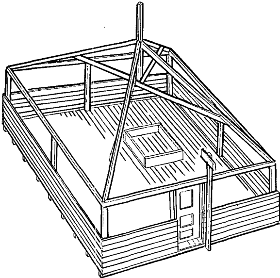
FIGURE 4.—Floor and frame for pyramidal tent.
