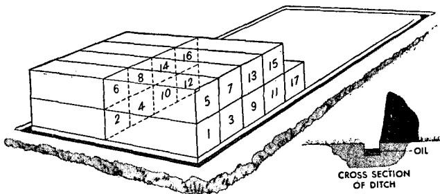
Figure 30. Compost pile.
