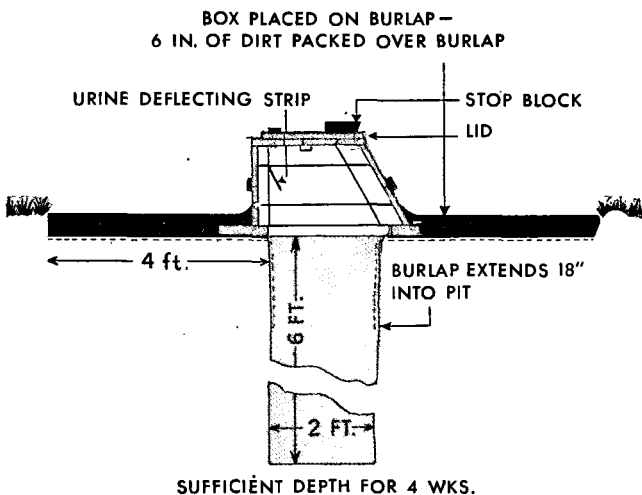
Figure 11. Deep pit latrine arrangement for 100 men.
