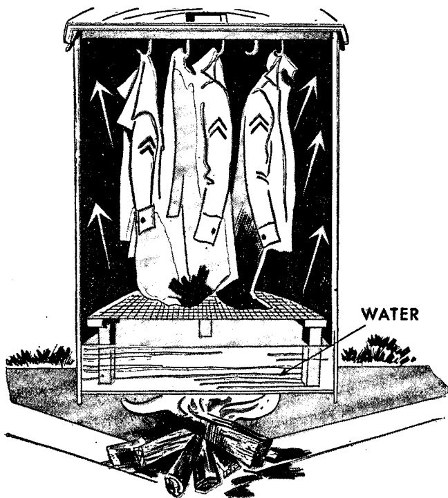
Figure 57. Serbian barrel disinfector (upward displacement of steam).
