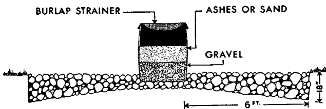
Figure 26. Soakage trench with barrel grease trap.
