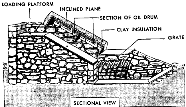
Figure 21. Inclined plane incinerator.
