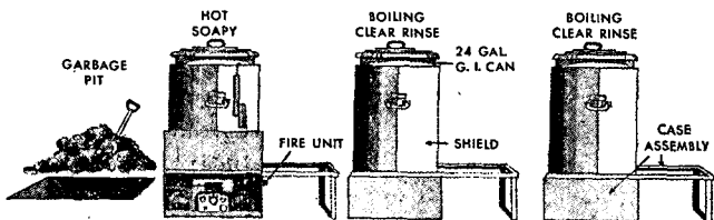
Figure 35. Mess kit, washing, using heater, water, range, field, M-1937.
